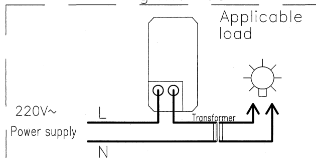
Wiring method
