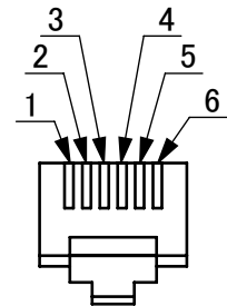
Pin assignment (2:1)
