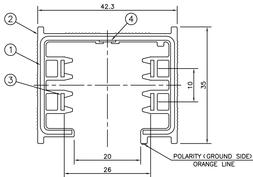
SECTIONAL VIEW OF TRACK
